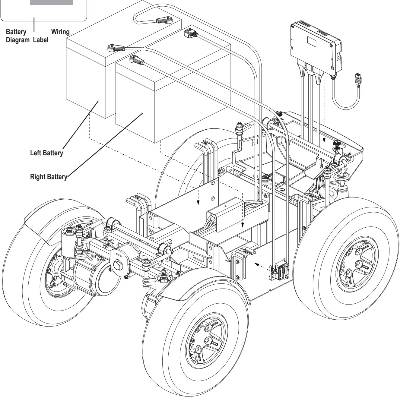
Figure 19. Battery Installation
