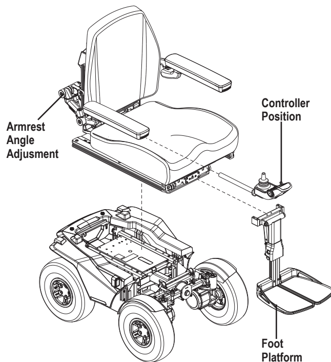
Figure 4. Assembly View
