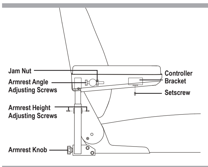
Figure 16. Seatback/Armrest Adjustment
